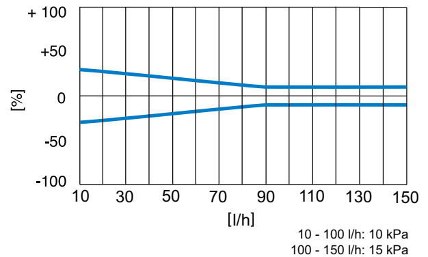
Flow tolerance
